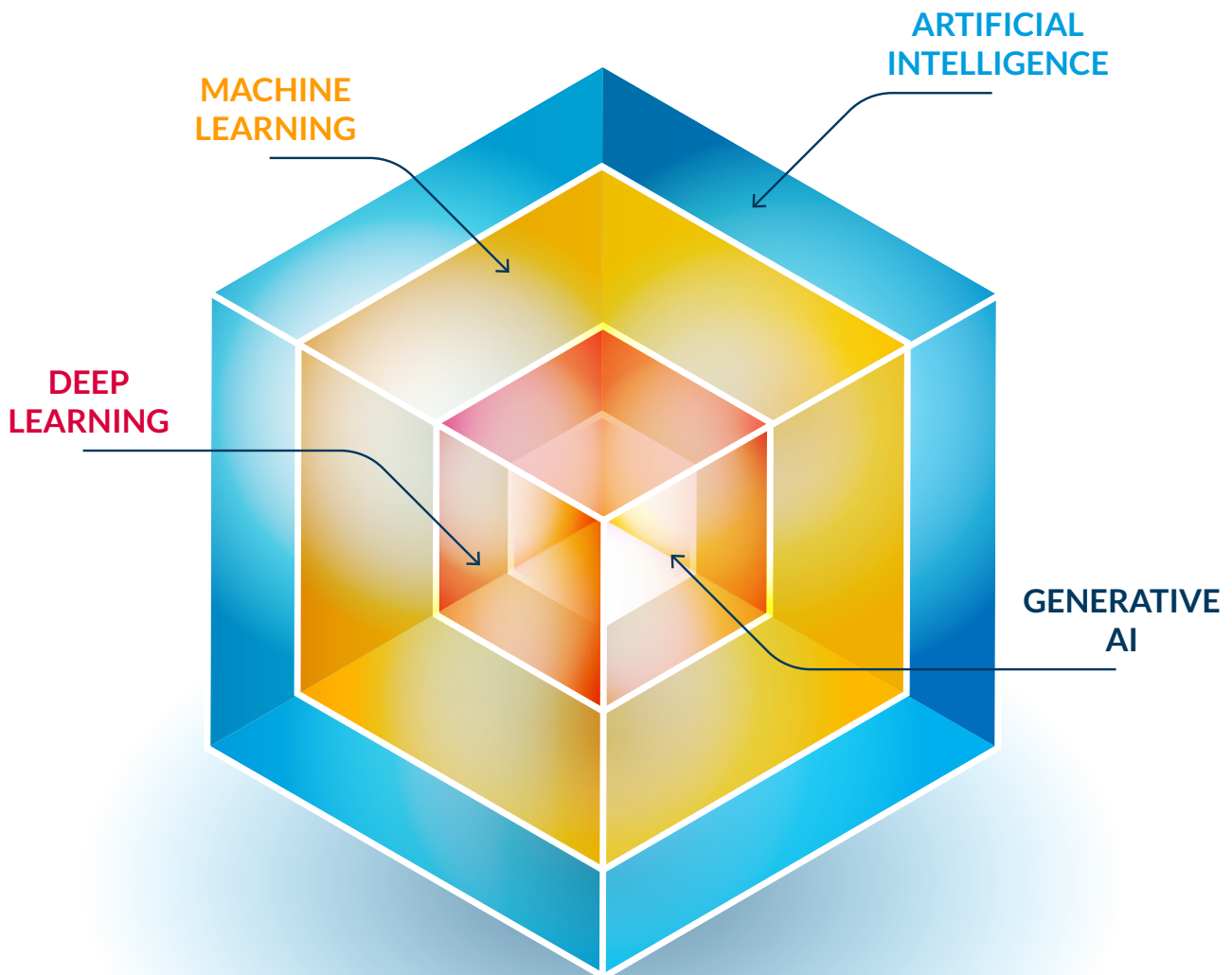
Figure 1 | AI terminology
